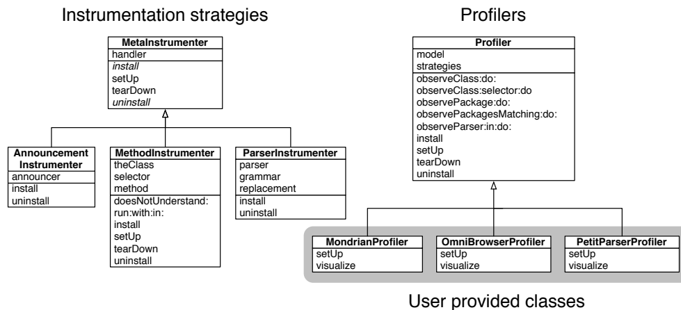
Figure 1 – The architecture of the MetaSpy profiler framework.
