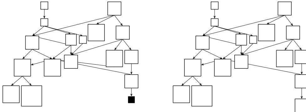
Figure 4 – Visualization of the production coverage of an XML grammar with uncovered productions highlighted in black (left); and the same XML grammar with updated test coverage and complete production coverage (right). The size of the nodes is proportional to the number of activations when running the test suite on the grammar.
