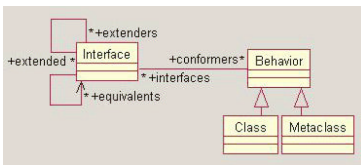
Figure 1: Relationships between Interfaces and Classes.
