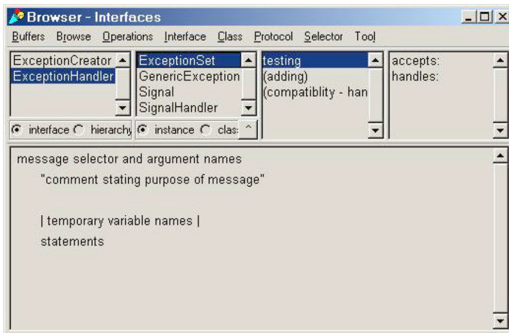
Figure 4: Interface views for classes implementing ExceptionHandler.
