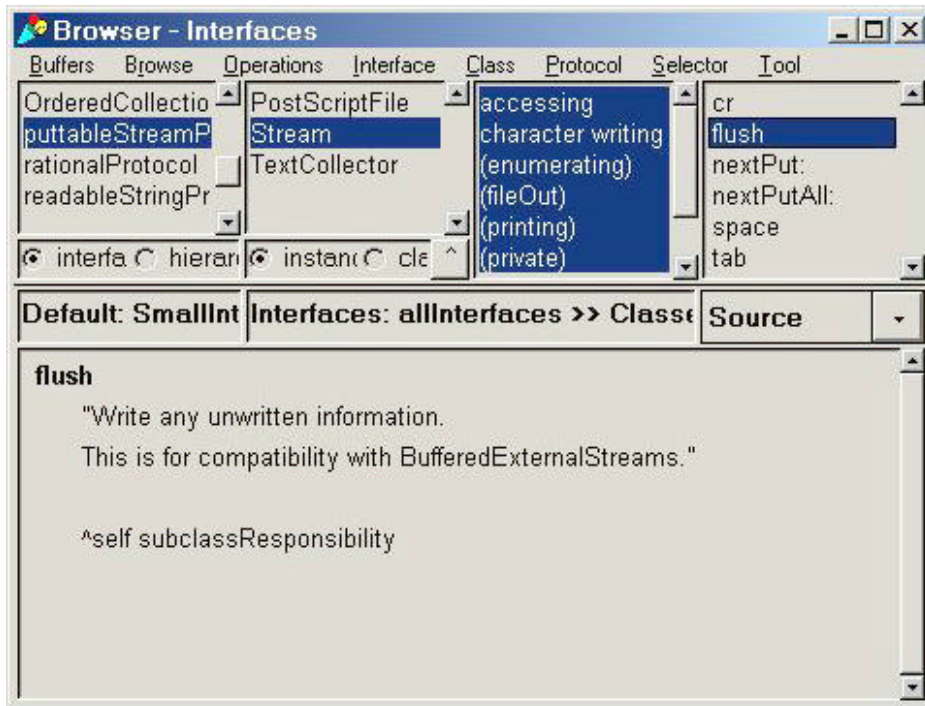
Figure 5: puttableStreamProtocol view of Stream.
