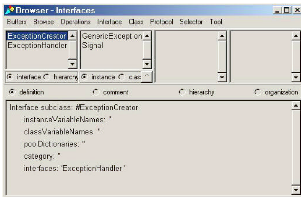
Figure 3: ExceptionCreator definition and classes implementing it.
