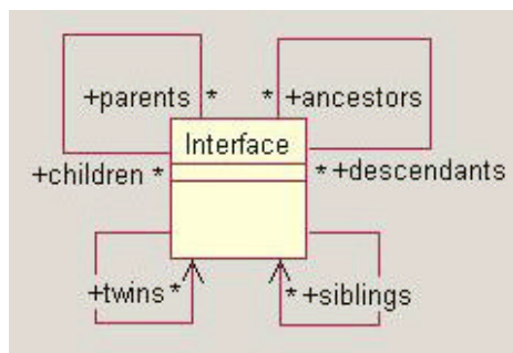
Figure 2: Relationships among Interfaces.
