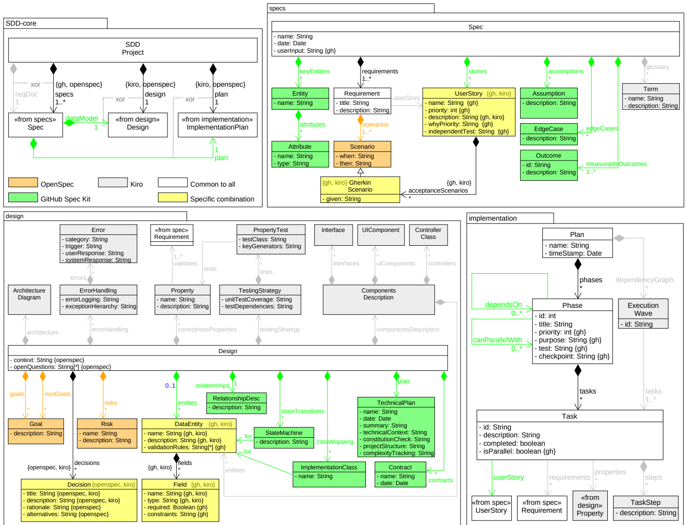
Figure 2 SDD metamodel based on GitHub Spec Kit, Kiro, and OpenSpec
