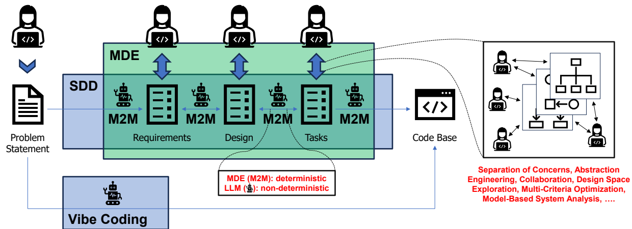
Figure 1 Commonalities and variabilities of vibe coding, SDD, and MDE
