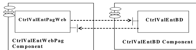
Figure 15: Component diagram: CORBA control components associated to the use case Login via Web
