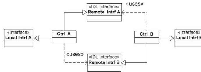
Figure 5: Control classes and their interfaces
