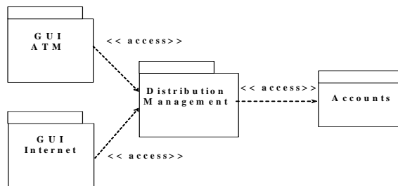
Figure 12: Analysis Packages
