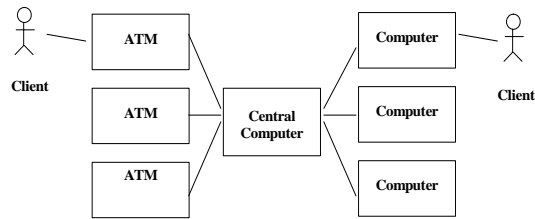
Figure 9: Banking system
