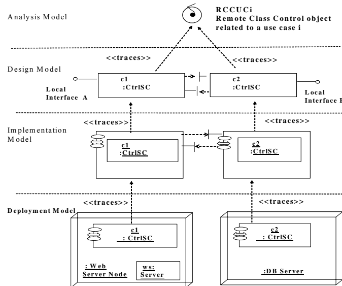
Figure 8: Traceability among the Analysis, Design, Implementation, and Deployment models related to the use case UCi
