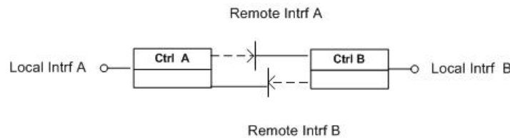
Figure 6: Another notation for IDL interfaces
