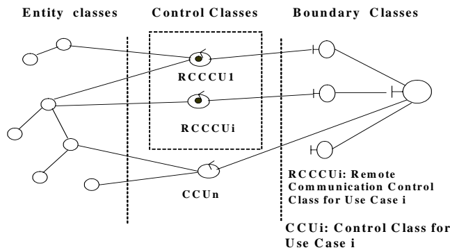
Figure 1: Class diagram related to thematic use cases
