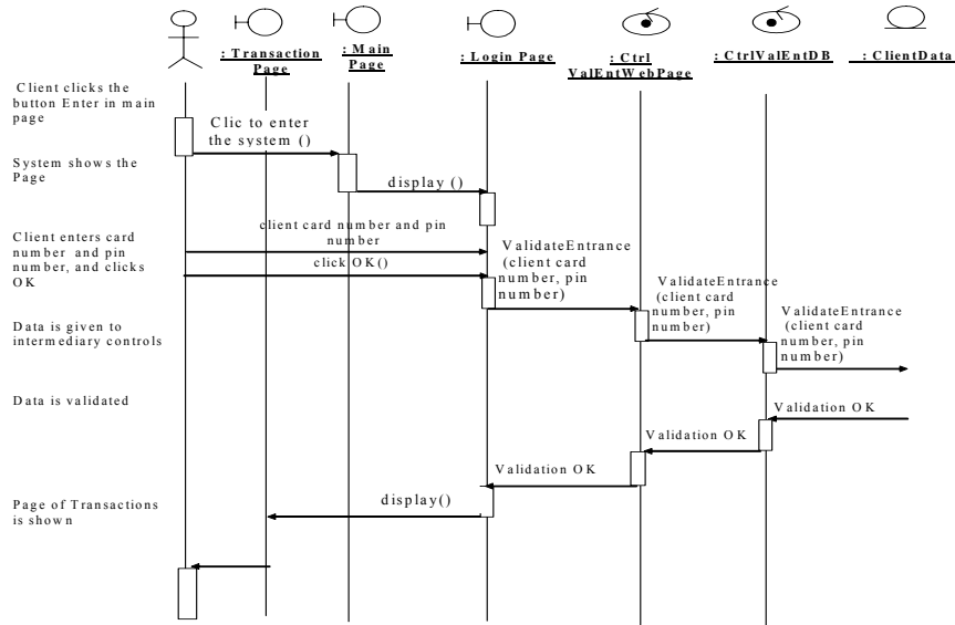
Figure 13: Sequence diagram for the use case Login via Web
