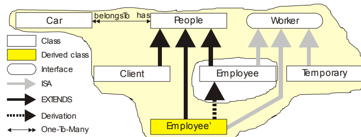
Fig. 2: Repository and external schema
