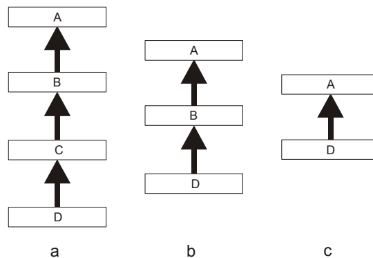
Fig. 4: Inheritance relationships depend on schemas
