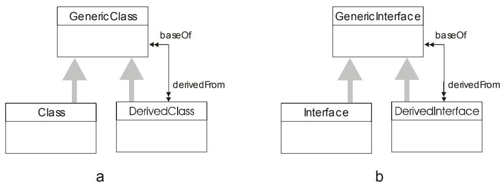
Fig. 3: a) Metadata for derived classes; b) Metadata for derived interfaces
