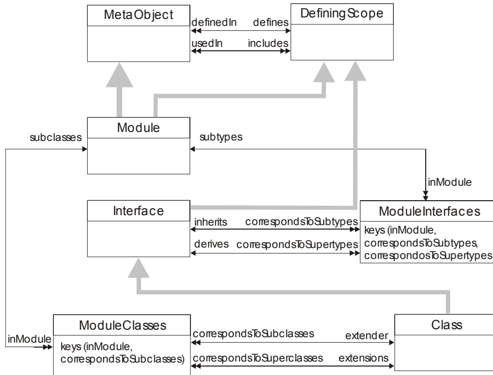
Fig. 5: Modelling the components of a schema as well as their relationships by schema
