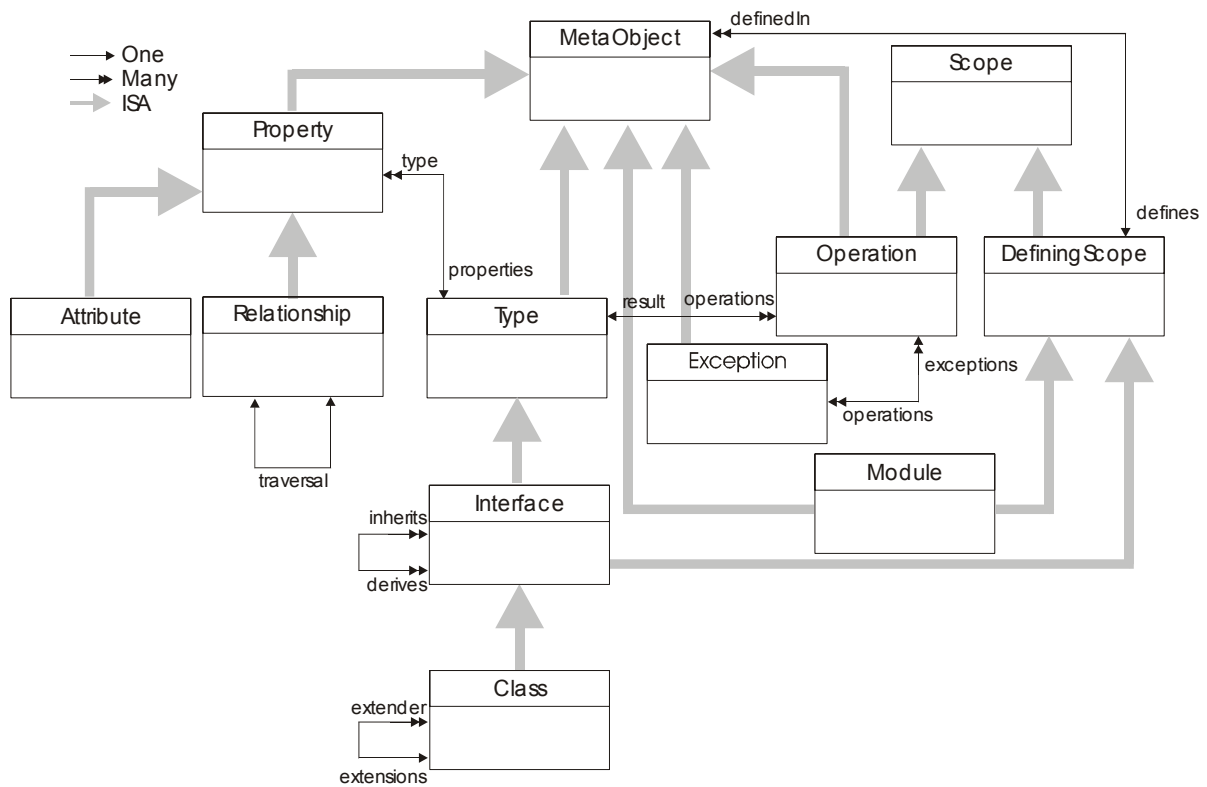
Fig. 1: An extract of the ODMG metaschema
