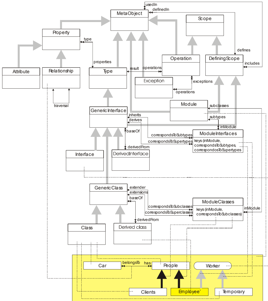
Fig. 6: Schema repository and an external schema definition
